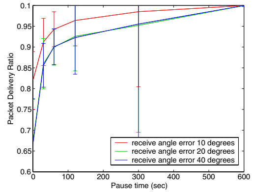
Figure 6. Packet Delivery Ratio for 5 flows transmitting across a partition
